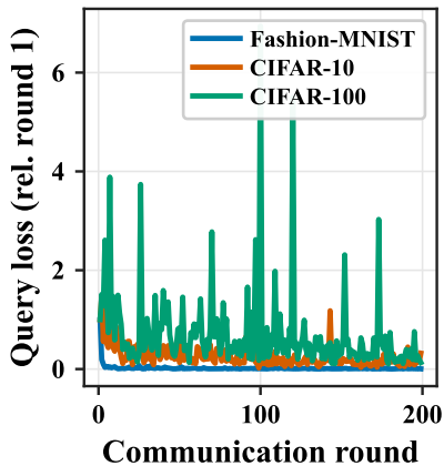
(b) Outer-loop convergence
