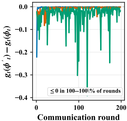
(a) Inner-step descent
