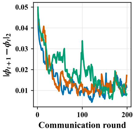
(c) Policy stabilization
